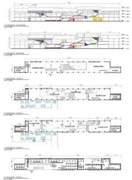
Floor Layout Plan and Zoning from Design Integration 2
